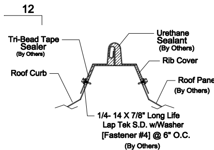
Rib Cover Attachment
