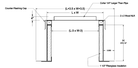
Pipe Curb with Collar PC SF
